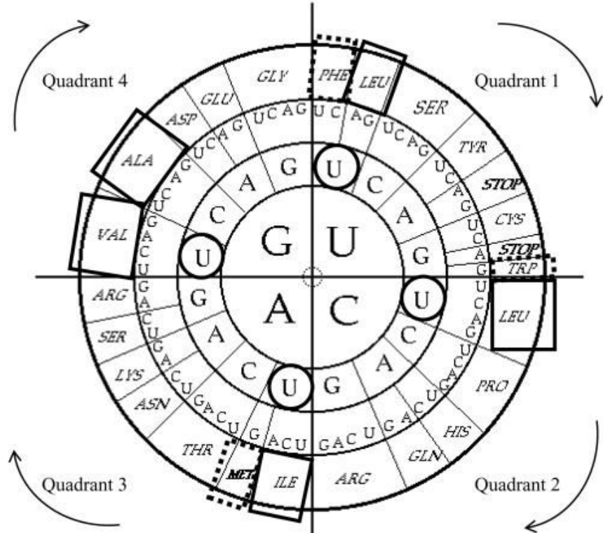
Rule 1. Same position in the four quadrants for essential hydrophobic codons (U at the center)
